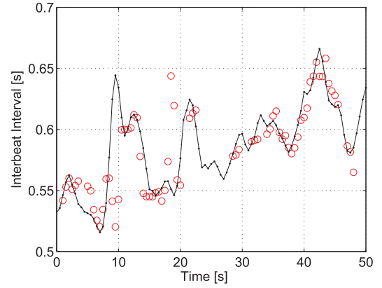
Fig. 21. Heart interbeat interval estimated from the output of the HPF and DCMP applied to s_B(t) when there is participant B only. The reference ECG data (black line) and radar measurement (red circles) are shown.
