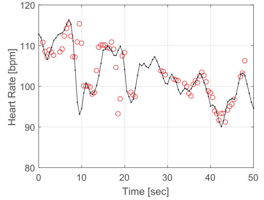
Fig. 25. Heart rate estimated from the output of the HPF and DCMP applied to s_B(t) when there is participant B only. The reference ECG data (black line) and radar measurement (red circles) are shown.
