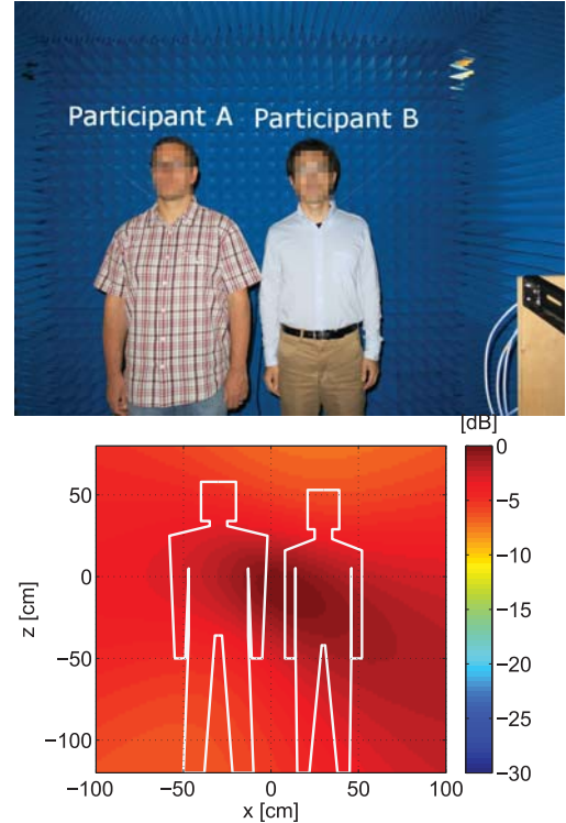
Fig. 7. Assumed scenario with two participants standing (top) and beamforming image obtained from the synthesized echoes of participants A and B (bottom).
