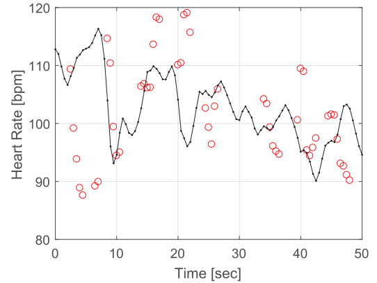
Fig. 26. Heart rate estimated from the output of the HPF applied to a single channel (ch1) of s_A(t) + s_B(t) when there are both participants A and B. The reference ECG data (black line) and radar measurement (red circles) are shown.
