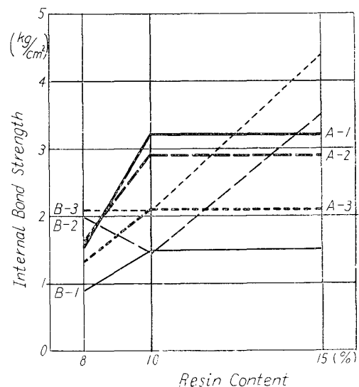
Fig. 3. Relations between resin content and internal bond strength.
