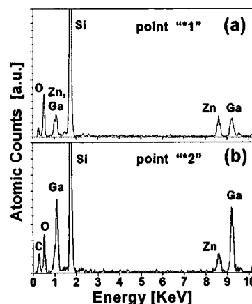
FIG. 9. (a) and (b) show \mu -EDX spectra recorded at the points marked as *1 and *2 in Fig. 8(b), respectively.
