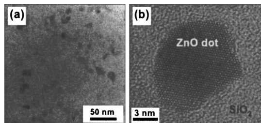
FIG. 12. (a) Plan-view TEM image of self-assembled ZnO nanodots on a \text{SiO}_2/\text{Si} substrate (dot density: 1.1 \times 10^{11} \text{ cm}^{-2} ) by MOCVD. The widths of the individual nanodots range from 5 to 15 nm (an average height of the nanodots is about 7 nm). (b) High-resolution TEM image of a self-assembled ZnO nanodot with a single-crystalline structure showing hexagonal atomic arrays.
