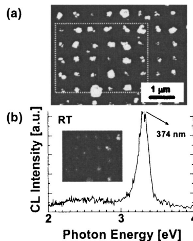
FIG. 5. (a) FE-SEM image of well-aligned ZnO clusters grown for 600 s. (b) CL spectrum of the FE-SEM image (a) measured at RT. The inset shows RT-CL image taken at the wavelength of 374 nm from the area designated as a dotted square in the FE-SEM image (a).
