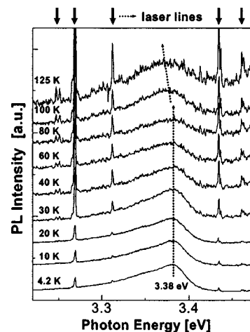
FIG. 13. Temperature-dependent \mu -PL spectra of 100 nanodots in the ZnO-nanodot sample presented at Fig. 2(a).
