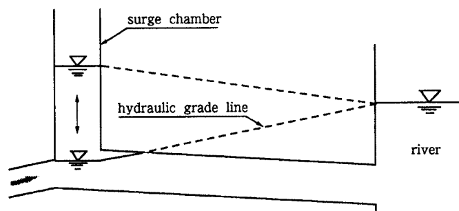
Fig. 1 Approximate graphical method for surging at initially full flowing tail-race tunnel [1].
