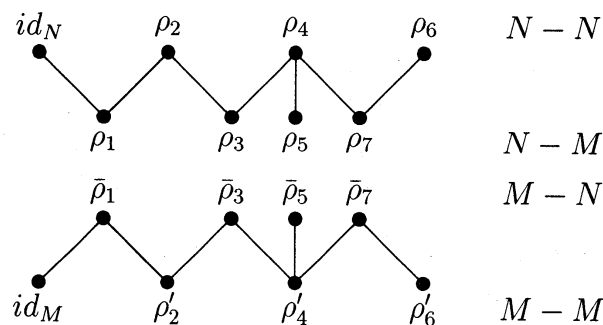
Figure 39: The (dual) principal graph E_8
