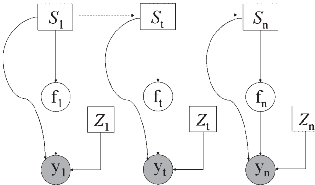
Figure 1 Dynamic Bayesian network representing a Factorial HMM. \mathbf{Z}_t 's are eventual exogenous variables that can be introduced in the model as explanatory variables.
