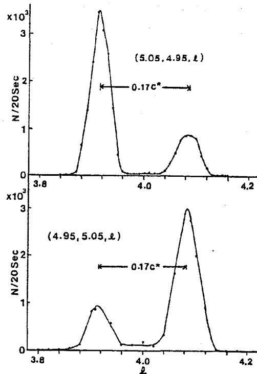
Fig.5 X-ray diffraction profiles of superlattice reflections along c^* at (5.05, 4.95, \ell ) and at (4.95, 5.05, \ell ).
