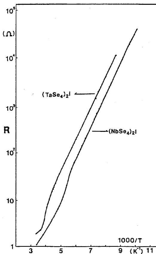
Fig.2 Temperature dependence of resistivity in (\text{MSe}_4)_2\text{I} , (M=Ta and Nb).
