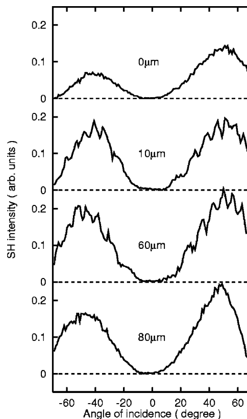
FIG. 4. Maker fringe patterns of the glass samples with cathode-side surface etchings of 0, 10, 60, and 80 \mu\text{m} .
