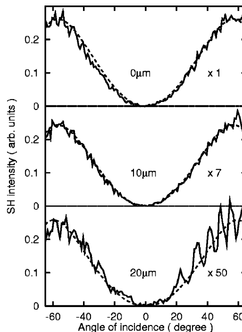
FIG. 5. Maker fringe patterns of the glass samples with anode-side surface etchings of 0, 10, and 20 \mu\text{m} . The dotted lines are the theoretical fringes drawn with the values shown in Tables I and II.
