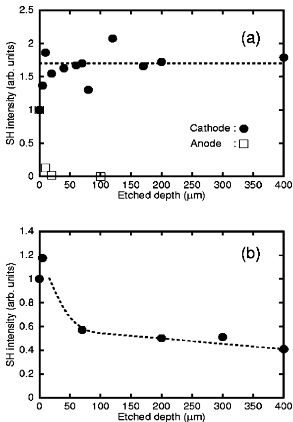
FIG. 3. Effects of (a) anode- and cathode-side surface etchings on the SH intensity and (b) cathode-side surface etching after 20 \mu\text{m} etching of the anode-side surface on the SH intensity. The intensity is normalized so that the intensity of 0- \mu\text{m} -etched sample is unity.
