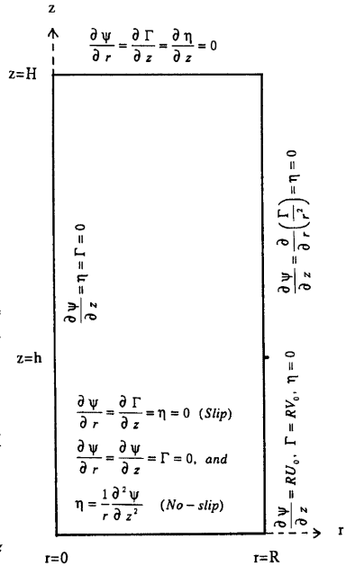
Fig. 2 Boundary conditions
