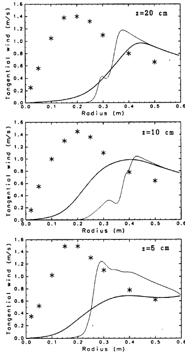
Fig. 7 Comparisons of the tangential wind at z = 5, 10 , and 20 cm. The thin and thick lines corresponds to CASE III (NSL \times 10 ) and CASE III (NSL \times 100 ), respectively.
