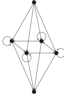
Figure 4: An example of a directed graph.
