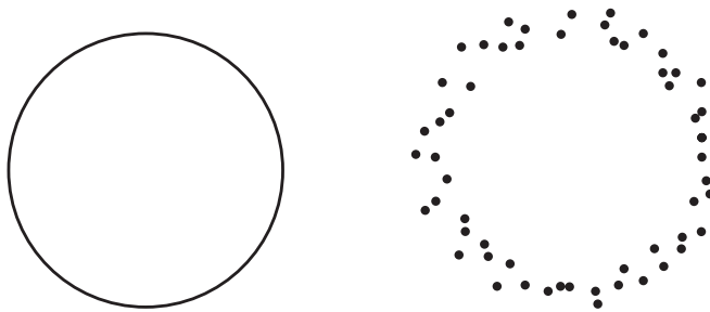
Figure 1: In the applications, we need a distance notion showing that a circle and a finite sample of it are similar even though the latter may contain small errors.
