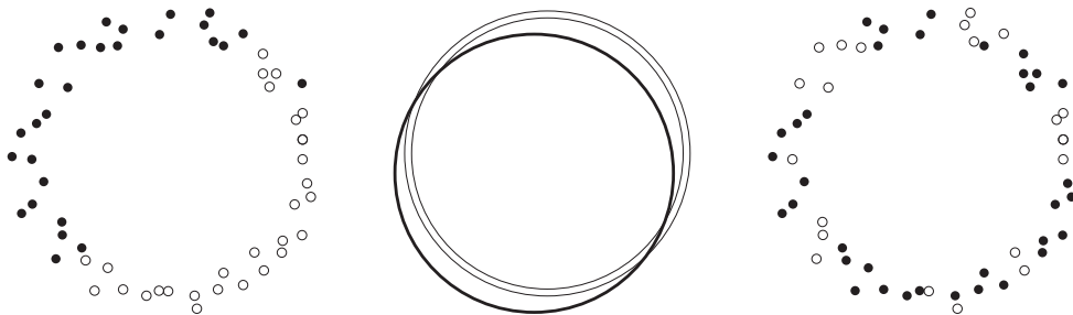
Figure 6: Three different datasets coloured in black and white showing different spatial configurations.
