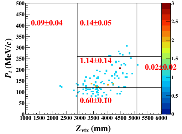
(b) K_L \rightarrow 3\pi^0 MC simulation
