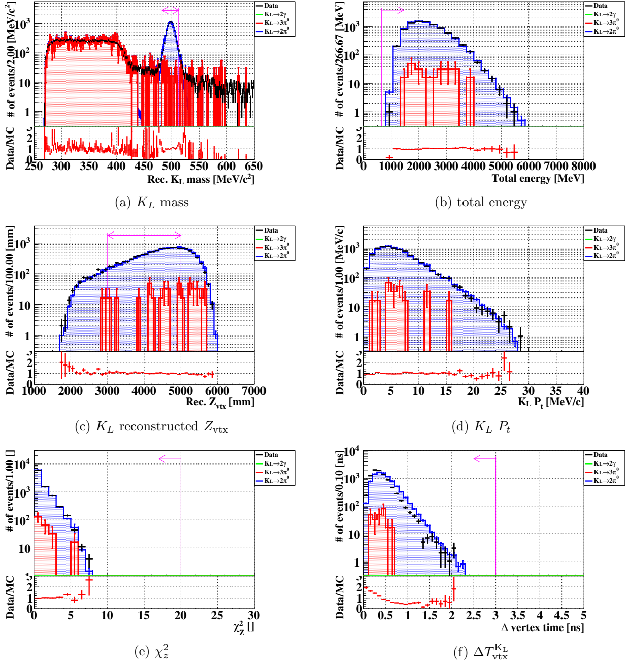
Figure 7.1: Distributions of the reconstructed K_L \rightarrow 2\pi^0 events for K_L mass (a), total energy (b), Z_{\text{vtx}}^{K_L} (c), K_L P_t (d), \chi_z^2 (e), and \Delta T_{\text{vtx}}^{K_L} after imposing cuts for K_L \rightarrow 2\pi^0 except for the cut of interest. Black points represent data. Red, blue, and green histograms represent MC simulations of K_L \rightarrow 3\pi^0 , K_L \rightarrow 2\pi^0 , and K_L \rightarrow 2\gamma , respectively. The contribution from K_L \rightarrow 2\gamma was negligibly small. Magenta lines show the accepted region. The data/MC ratios are shown below each panel. The error bars represent statistical errors.
