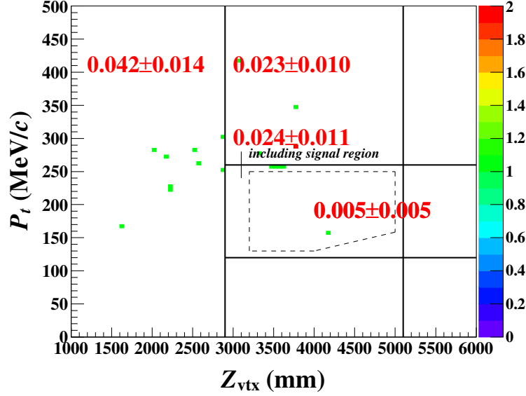
Figure 8.9: P_t vs. Z_{\text{vtx}} of the events after imposing the K_L \rightarrow \pi^0 \nu \bar{\nu} selection criteria on the beam-core K_L \rightarrow 2\gamma MC events.
