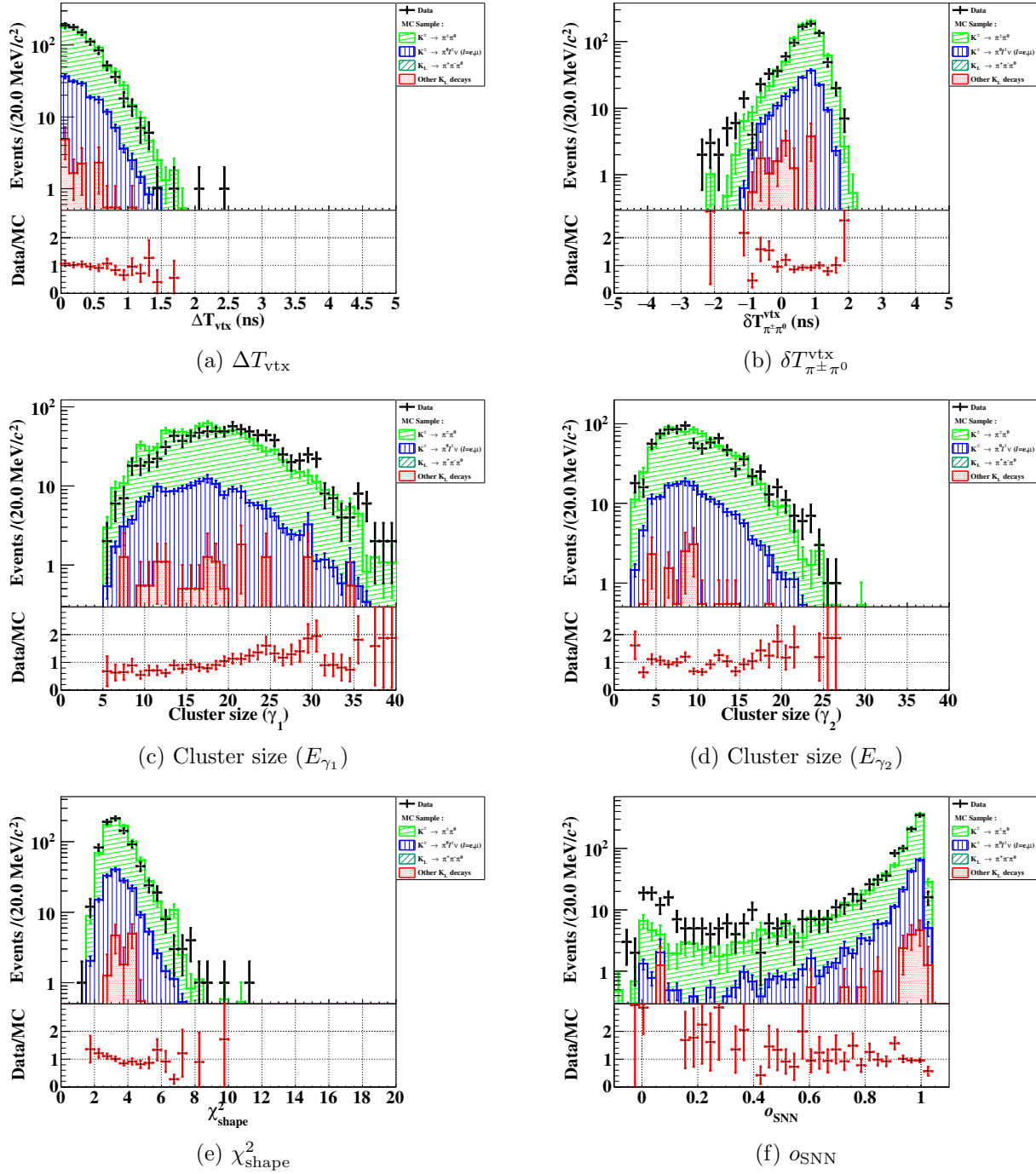
Figure 8.24: Distributions of \Delta T_{\text{vtx}} (a), \delta T_{\pi^\pm \pi^0}^{\text{vtx}} (b), Cluster size ( E_{\gamma_1} ) (c), Cluster size ( E_{\gamma_2} ) (d), larger \chi^2_{\text{shape}} between photon clusters (e), and smaller o_{\text{SNN}} between photon clusters (f) for K^\pm \rightarrow \pi^\pm \pi^0 events after imposing cuts except for the one of interest. Black points represent data. The colored histograms represent MC events (stacked). Light-green, blue, and green histograms represent K^\pm \rightarrow \pi^\pm \pi^0 , K^\pm \rightarrow \pi^0 \ell^\pm \nu ( \ell = e, \mu ) and K_L \rightarrow \pi^+ \pi^- \pi^0 MC, respectively. Red histograms represent MC simulations of other K_L decays ( K_L \rightarrow \pi^\pm e^\mp \nu , K_L \rightarrow \pi^\pm \mu^\mp \nu , K_L \rightarrow 2\pi^0 , K_L \rightarrow \pi^\pm e^\mp \nu \gamma , K_L \rightarrow \pi^0 \pi^\pm e^\mp \nu_e ). The data/MC ratios are shown below each panel. The error bars represent statistical errors.
