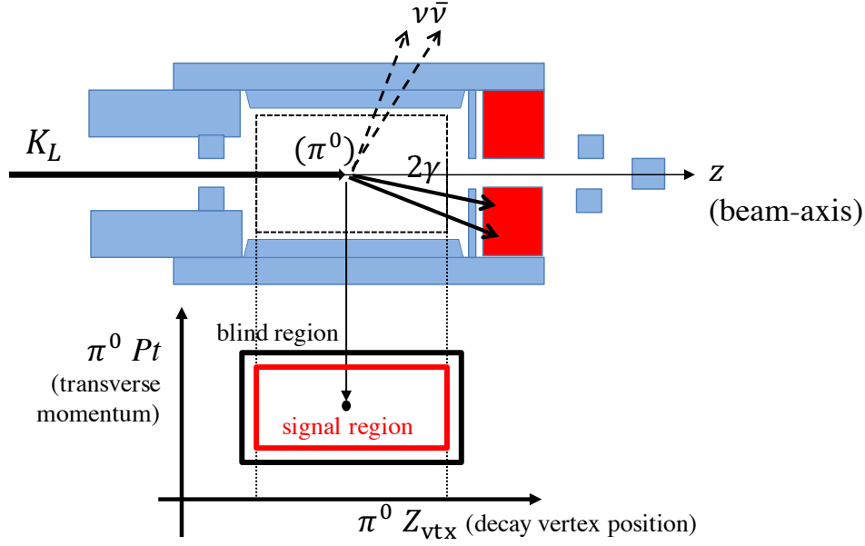
Figure 2.3: Schematic view of the opening angle between the two photons and Z_{\text{vtx}} .
