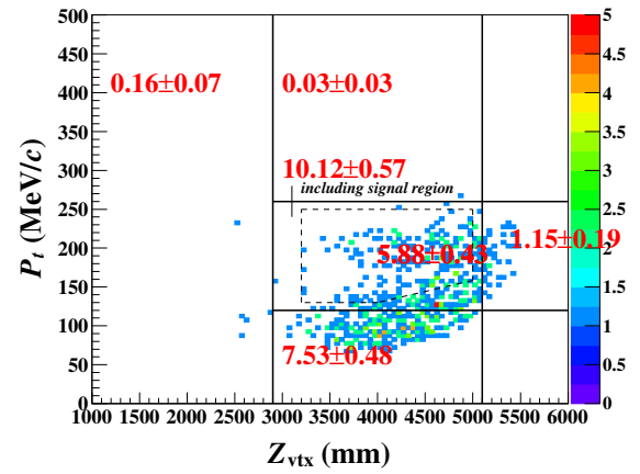
(b) K_L \rightarrow 2\pi^0 MC simulation
