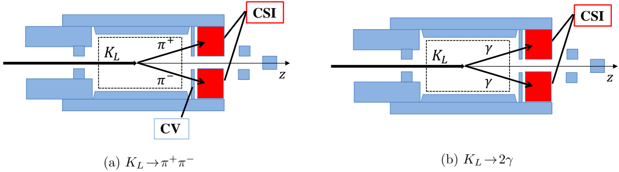
Figure 2.6: Schematic views of the K_L \rightarrow \pi^+ \pi^- (left) and the K_L \rightarrow 2\gamma (right) decay.
