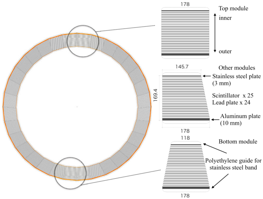
Figure 2.21: Cross-sectional views of IB (left) and a IB module (right). The figures are quoted from Ref. [47]. Scales in the figures are in units of mm.
