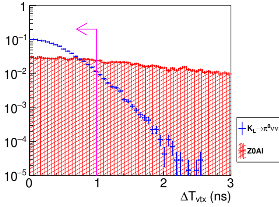
Figure 7.16: Distribution of \Delta T_{vtx} for the data taken in Z0A1 run (red) and K_L \rightarrow \pi^0 \nu \bar{\nu} MC events (blue). The magenta line and arrow represent the accepted region of the signal.
