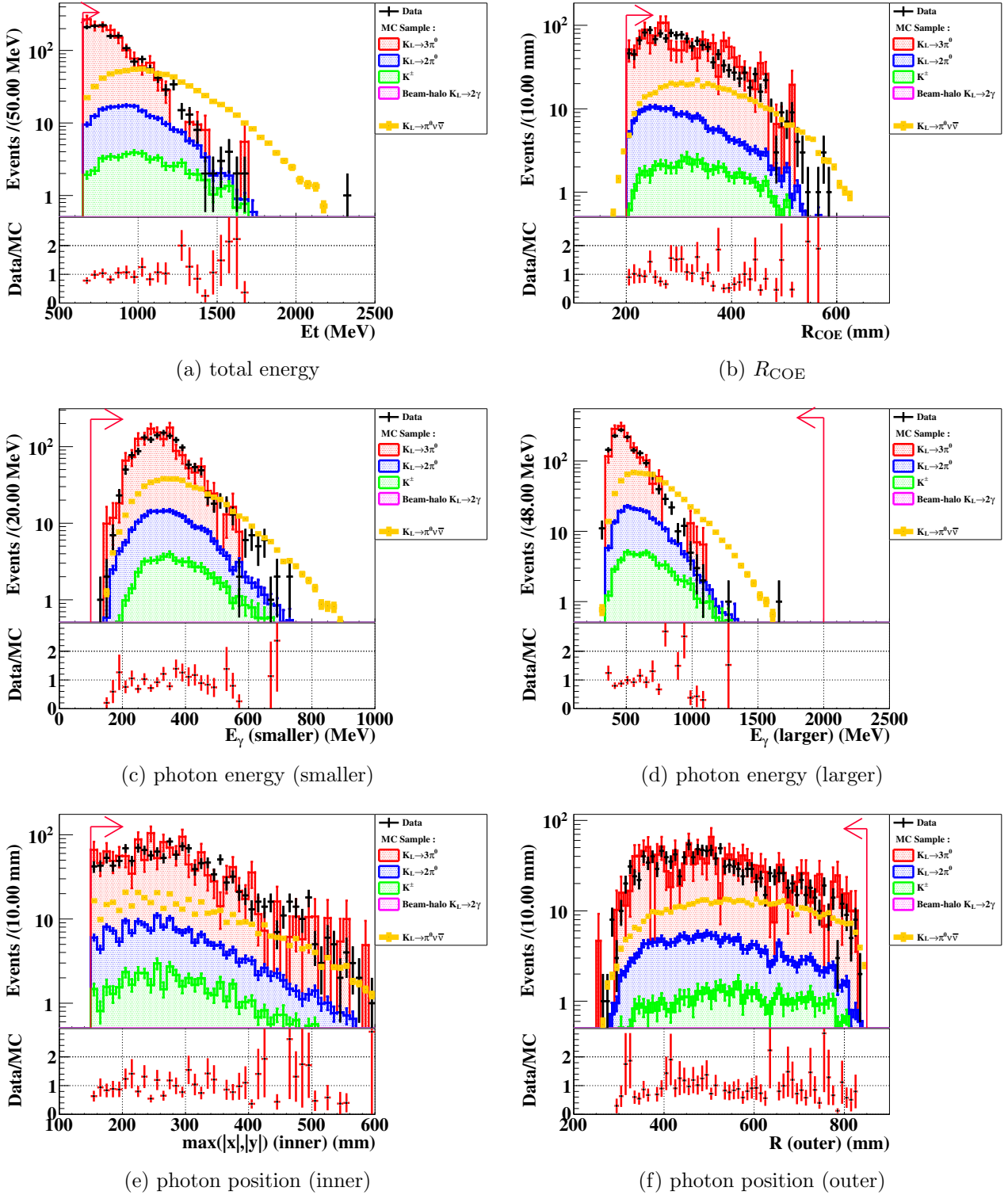
Figure 7.10: Distributions of the total energy (a), R_{\text{COE}} (b), smaller photon energy (c), larger photon energy (d), inner photon position (e), and outer photon position (f) under a loose cut condition in the blind region. The black histograms represent the data. The red, blue, green, and magenta histograms represent MC simulations of K_L \rightarrow 3\pi^0 , K_L \rightarrow 2\pi^0 , K^\pm , and beam-halo K_L \rightarrow 2\gamma decays, respectively. The number of events in the MC simulation except for K_L \rightarrow \pi^0 \nu \bar{\nu} was normalized with K_L yield. The orange histograms represent the K_L \rightarrow \pi^0 \nu \bar{\nu} MC, whose vertical axis is in arbitrary units. All the trigger-related cuts and photon-selection cuts are applied on the data and the K_L \rightarrow 3\pi^0 and K_L \rightarrow 2\pi^0 MC, whereas they are not applied on the K_L \rightarrow \pi^0 \nu \bar{\nu} MC. Besides, the other kinematic cuts are applied except for the cuts of interest. For the veto cuts, the energy thresholds of IB and MB are loosened to 10 MeV, and veto cuts on IBCV and MBCV are not applied. The pink lines and arrows indicate the region accepted by the cuts.
