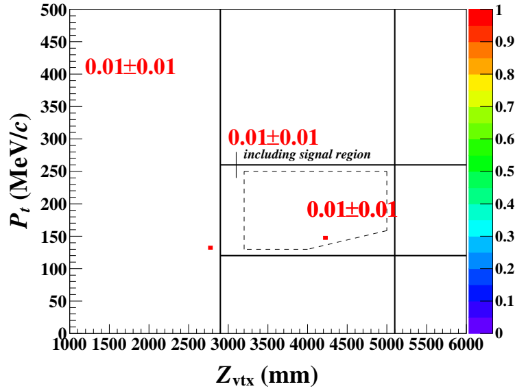
Figure 8.10: P_t vs. Z_{\text{vtx}} of the events after imposing the K_L \rightarrow \pi^0 \nu \bar{\nu} selection criteria on the K_L \rightarrow 3\pi^0 MC events.
