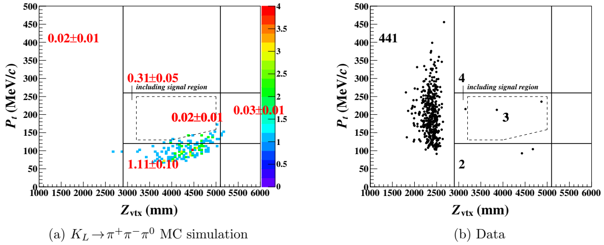
Figure 8.1: P_t vs. Z_{\text{vtx}} of the events after imposing the K_L \rightarrow \pi^0 \nu \bar{\nu} selection criteria except for CSD- \pi^+ \pi^- \pi^0 on the K_L \rightarrow \pi^+ \pi^- \pi^0 MC events (a) and data (b). The numbers indicate the number of background events in each different region. Although the actual P_t from K_L \rightarrow \pi^+ \pi^- \pi^0 decay is lower than 132 MeV/c due to the kinematical limit, the reconstructed P_t can be large when K_L \rightarrow \pi^+ \pi^- \pi^0 decays occur off the beam-axis near CSI. For the K_L \rightarrow \pi^+ \pi^- \pi^0 MC simulation, we simulated 8.0 \times 10^{13} K_L \rightarrow \pi^+ \pi^- \pi^0 events, which correspond to 9 \times 10^1 times higher statistics than data. In this cut set, contributions from other background sources were expected to be 0.79 \pm 0.20 events in the region of 2900 < Z_{\text{vtx}} < 5100 mm and P_t < 120 MeV/c.
