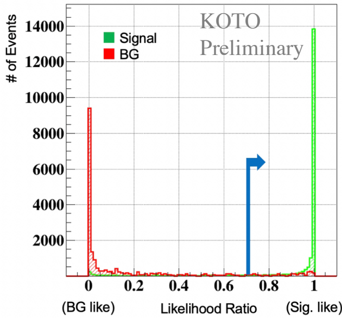
Figure 10.3: Likelihood ratio distributions. The green and red histograms show the K_L \rightarrow \pi^0 \nu \bar{\nu} and beam-halo K_L \rightarrow 2\gamma MC events, respectively. The blue arrow shows the threshold to maintain the signal acceptance of 90%. This figure is quoted from Ref. [71].
