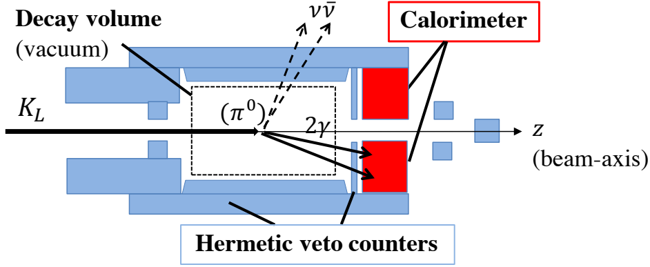
Figure 2.1: Schematic view of the signal detection in KOTO. The \pi^0 from the K_L \rightarrow \pi^0 \nu \bar{\nu} decay immediately decays into two photons. We detect the two photons from the \pi^0 decay with a calorimeter, and ensure that there are no other detectable particles by hermetic veto counters surrounding the decay volume.
