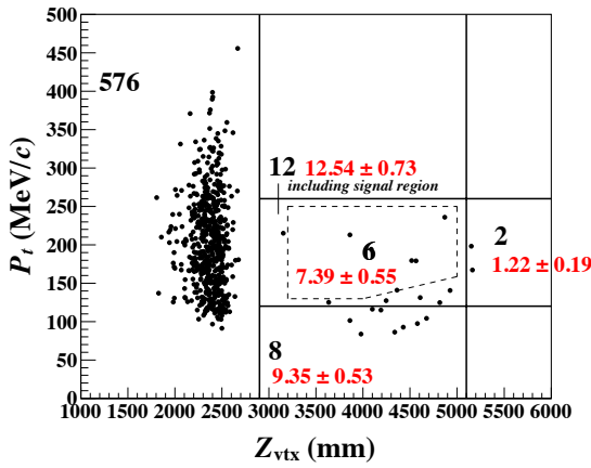
(a) Data
