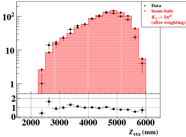
(a) Z_{\text{vtx}}
