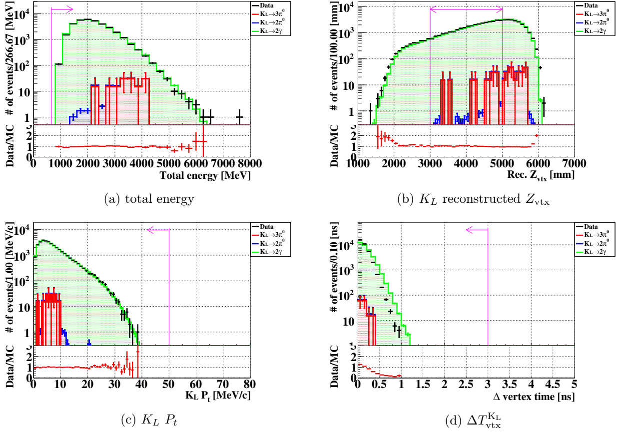
Figure 7.4: Distributions of reconstructed K_L \rightarrow 2\gamma events for total energy (a), Z_{\text{vtx}}^{K_L} (b), K_L P_t (c), and \Delta T_{\text{vtx}}^{K_L} (d) after imposing cuts for K_L \rightarrow 2\gamma except for the cut of interest. The meaning of the black points, colors of histograms, lines in magenta, below panel, and error bars are the same as for Fig. 7.1.
