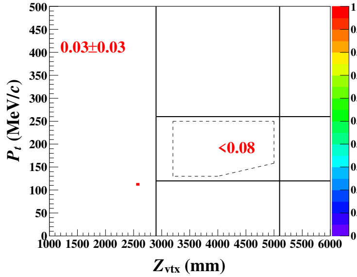
Figure 8.6: P_t vs. Z_{\text{vtx}} of the events after imposing the K_L \rightarrow \pi^0 \nu \bar{\nu} selection criteria on the K_L \rightarrow 2\pi^0 MC events. The upper limit on the number is at the 90% confidence level.
