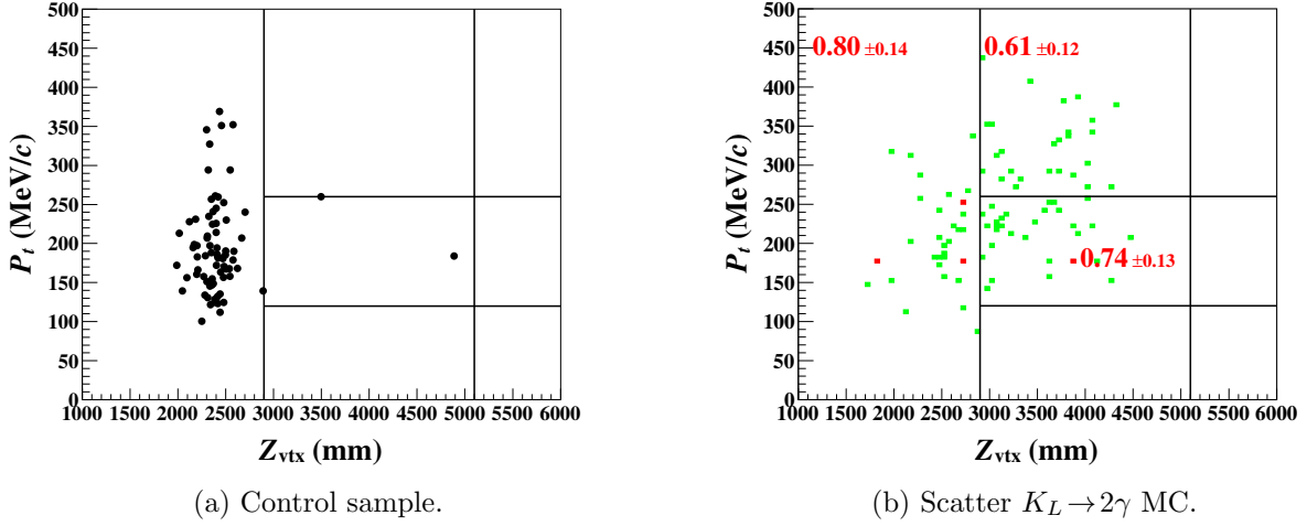
Figure 8.17: P_t vs. Z_{\text{vtx}} after imposing CSD-Had, CSD- \eta , and PSD-FFT cuts on the events in Fig. 8.13b (left) and events in the scattering K_L \rightarrow 2\gamma MC simulation (right). The numbers in red indicate the number of events in each region bounded by lines. The number of events in the MC simulation is normalized with the number of collected K_L 's in the Z0Al run.
