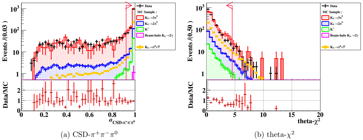
Figure 7.22: Distributions of o_{\text{CSD-}\pi^+\pi^-\pi^0} (left) and \chi_{\theta}^2 (right) under a loose veto cut condition in the blind region. The veto cut condition and the meaning of the colors of histograms and lines in pink are the same as for Fig. 7.10.
