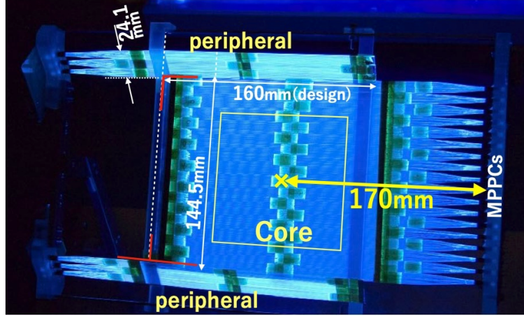
Figure 10.1: Picture of UCV (provided by K.Kotera.)
