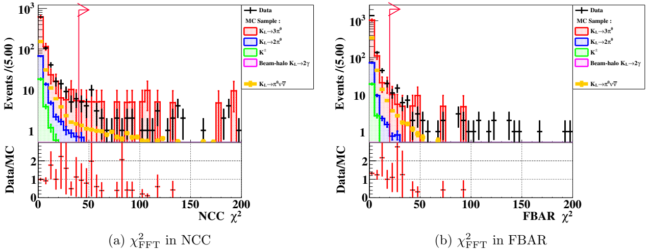
Figure 7.20: Distributions of \chi^2_{\text{FFT}} in NCC (left) and FBAR (right) under a loose cut condition in the blind region. In the loose cut condition, the energy thresholds of IB and MB are loosened to 10 MeV, and veto cuts on IBCV and MBCV are not applied. Besides, the energy threshold of NCC (FBAR) is loosened to 10 MeV in the NCC (FBAR) FTT- \chi^2 distribution. The meaning of the colors of histograms and lines in pink are the same as for Fig. 7.10.
