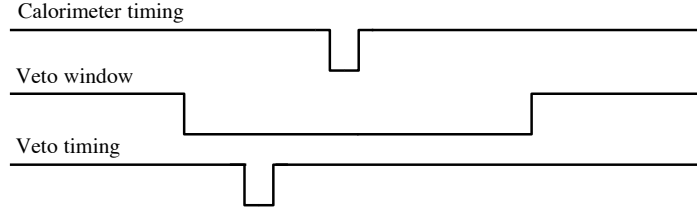
Figure 2.11: Schematic view of a veto window and timings measured with the calorimeter and veto counters.
