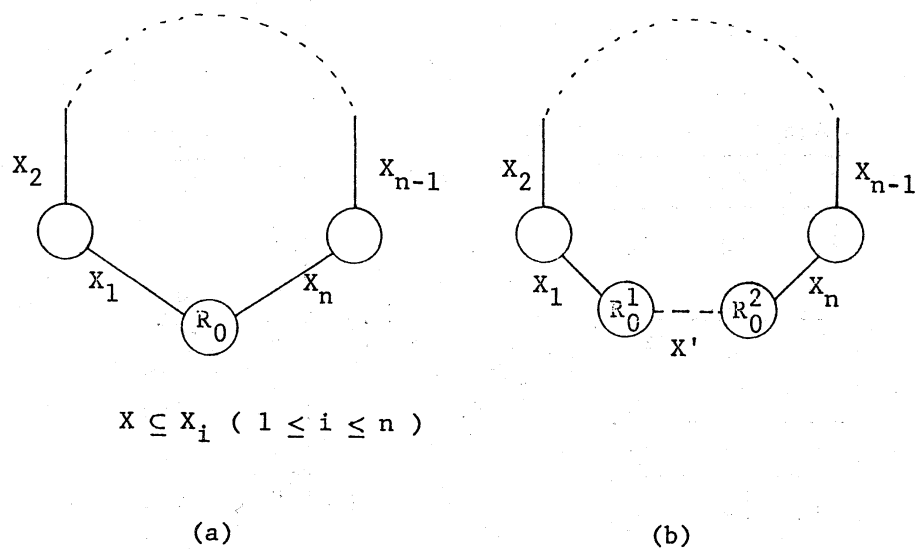
Fig.11 Removal of a cycle by an MVD-based decomposition
