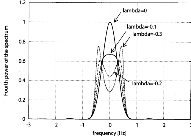
Figure 3: The variances of cross-interference of signature waveforms using i.i.d. codes ( \lambda = 0 ) and Markov codes ( \lambda = -0.1, -0.2 and -0.3 ) are, respectively, equal to the areas under the corresponding curves.
