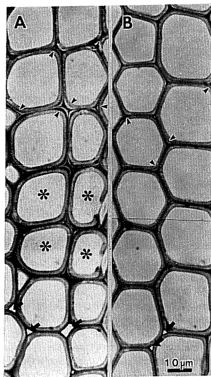
Fig. 4 Characters of tracheids contained in a compression wood are of 2-day inclination (A) and 1-day inclination (B) in SUGI. The arc of A is composed of some tracheids having various characters of compression wood, namely, "intercellular space (thick arrows)", "thick and highly-lignified secondary wall (asterisks)", and "faint lignin-rich layer between S_1 and S_2 (arrow heads)". These characters are weaker in B. Cells having the faint lignin-rich layer at the cell corner (see arrow heads) were used as the marker cell.
