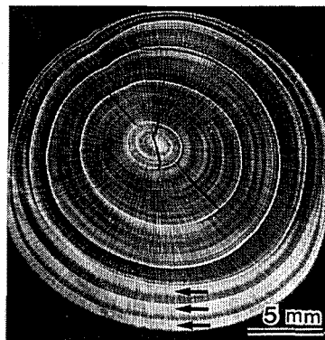
Fig. 3 Overall view of a stem section at 1.5 m from the top in a tree of HINOKI which was treated three times by one month inclination. The current annual ring has three compression wood arcs at the lower-side of inclination (arrows).
