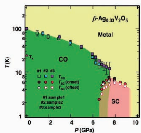
図1 \beta\text{-Ag}_{0.33}\text{V}_2\text{O}_5 の圧力温度相図. [2]
