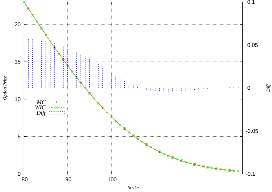
Figure 5: Complex basket option prices that contains of 6 underlying assets. MC means the option prices calculated by Monte Carlo simulation, while WIC indicates the approximate prices calculated by the formula given in Theorem 4.2. The CPU time to calculate our results (WIC) was 2.612 seconds for each case in average.
