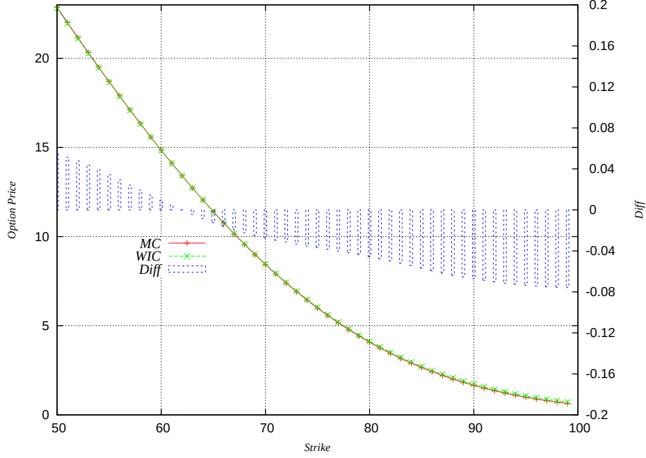
Figure 4: Basket option prices for the calibrated parameters. MC and WIC indicate Monte Carlo simulation and our approximation results, respectively. The other parameters are set as r_d(t) = 0.00977 , r_{1,f}(t) = 0.0222 , r_{2,f}(t) = 0.04848 , S_{1,0} = 77.54 , S_{2,0} = 78.60 , T = 3 and w_1 = w_2 = 0.5 . The correlation between them is set as \rho = 0.5 .
