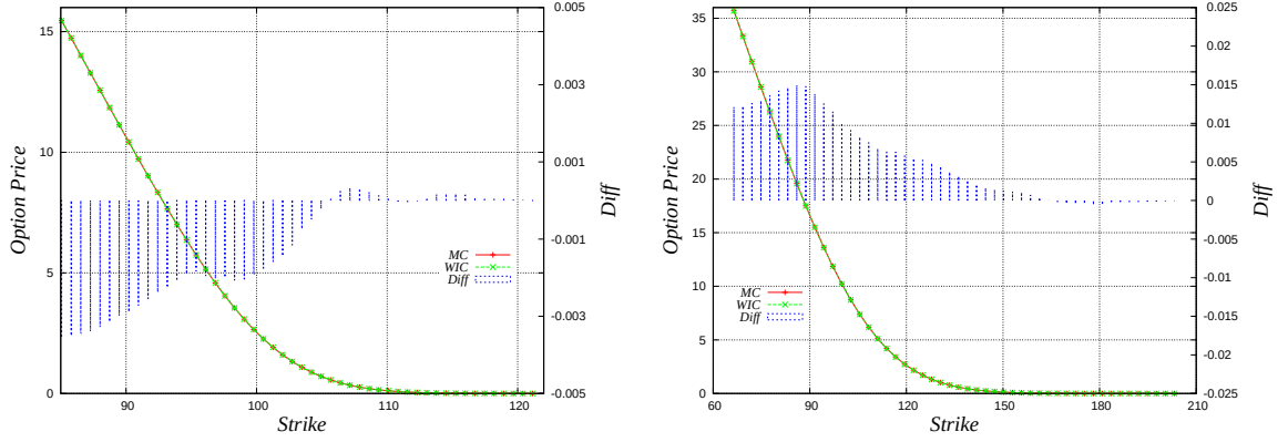
Figure 1: Asian option prices for the square-root model. The left-hand side panel corresponds to the short maturity ( T = 6 months) case and the right-hand side panel corresponds to the long maturity ( T = 5 years) case. MC means the option prices calculated by Monte Carlo simulation, while WIC indicates the approximate prices calculated by the formula given in Theorem 4.2. The parameters are set as S_0 = 100 , r = 0.03 , and \sigma = 1.33 .
