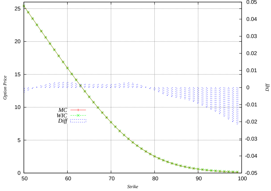
Figure 3: Asian option prices for the calibrated parameters. MC indicates the results calculated by Monte Carlo simulation, while WIC means that the results are obtained our approximation method. The other parameters are set as r_d(t) = 0.00977 , r_{1,f}(t) = 0.0222 , S_{1,0} = 77.54 , T = 3 .
