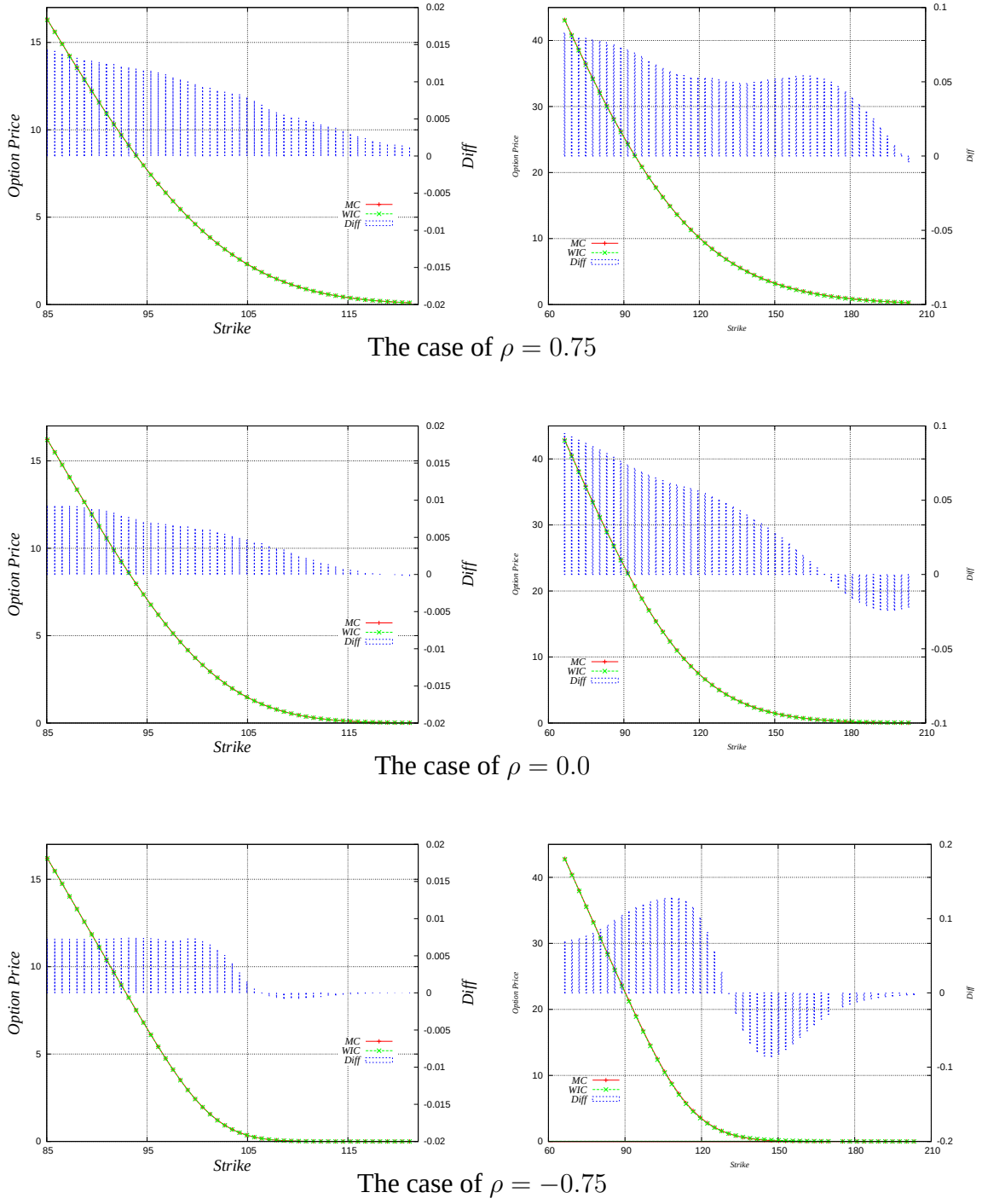
Figure 2: Basket option prices for the CEV model. The left-hand side panel corresponds to the short maturity ( T = 6 months) case and the right-hand side panel corresponds to the long maturity ( T = 5 years) case. The top two panels report the results for the case of \rho = 0.75 , the middle panels \rho = 0 and the bottom panels \rho = -0.75 , respectively. MC means the option prices calculated by Monte Carlo simulation, while WIC indicates the approximate prices calculated by the formula given in Theorem 4.2. The parameters are set as S_{1,0} = S_{2,0} = 100 , r = 0.03 , \beta_1 = 1 , \beta_2 = 0.5 , \sigma_1 = 0.15 and \sigma_2 = 1.33 .
