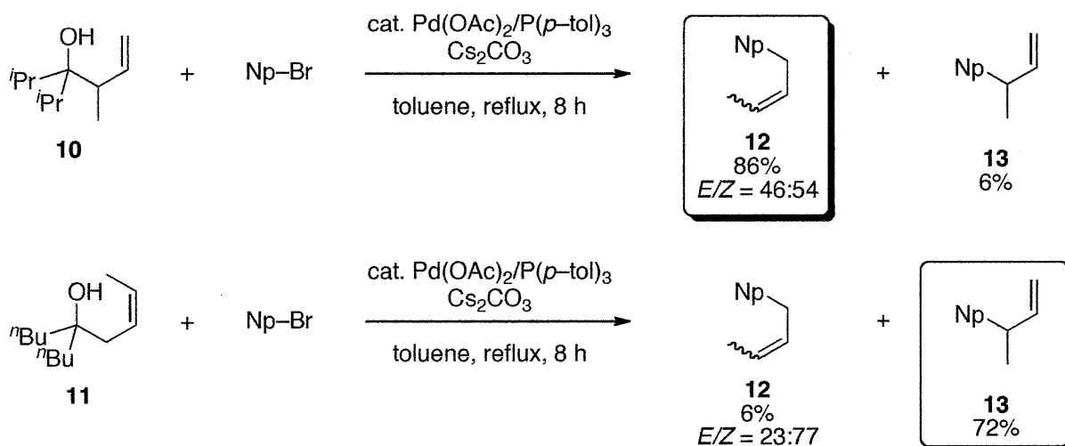
Scheme 12.
