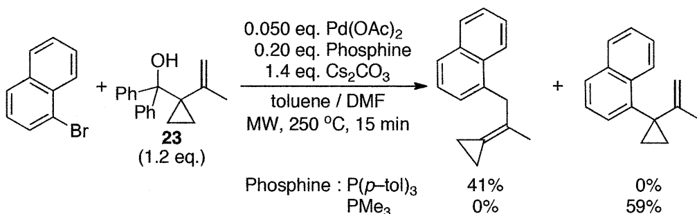
Scheme 32.
