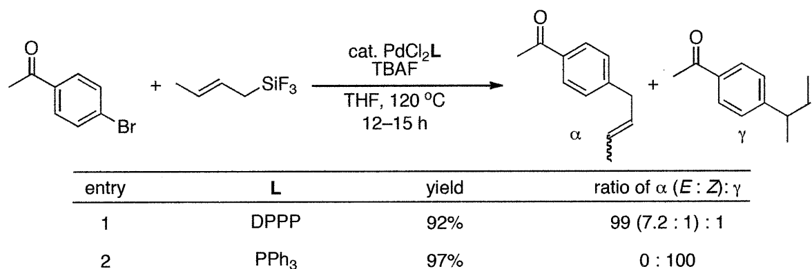
Scheme 5.
