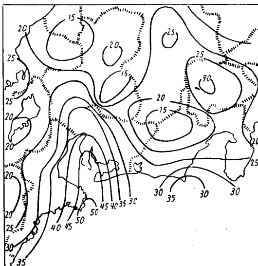
Fig. 1 The distributions of the maximum ten minute wind velocities
