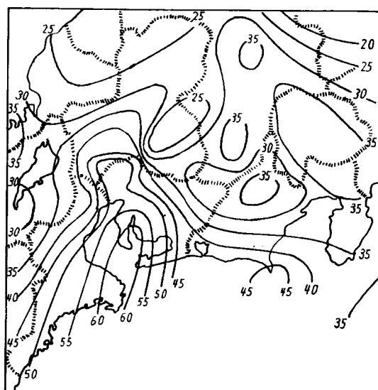
Fig. 2 The distributions of the maximum wind velocities
