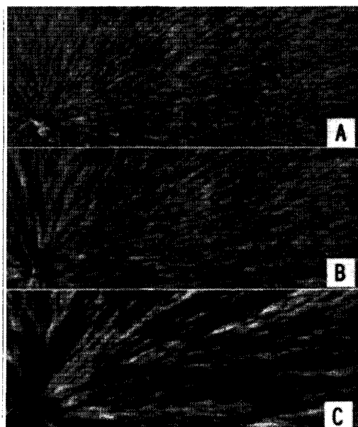
Figure1: POM images of the spherulites of poly(butene-1). Width of the images is 200\ \mu\text{m} . Crystallization temperatures are A : 85^{\circ}\text{C} , B : 90^{\circ}\text{C} , and C : 96^{\circ}\text{C} .
