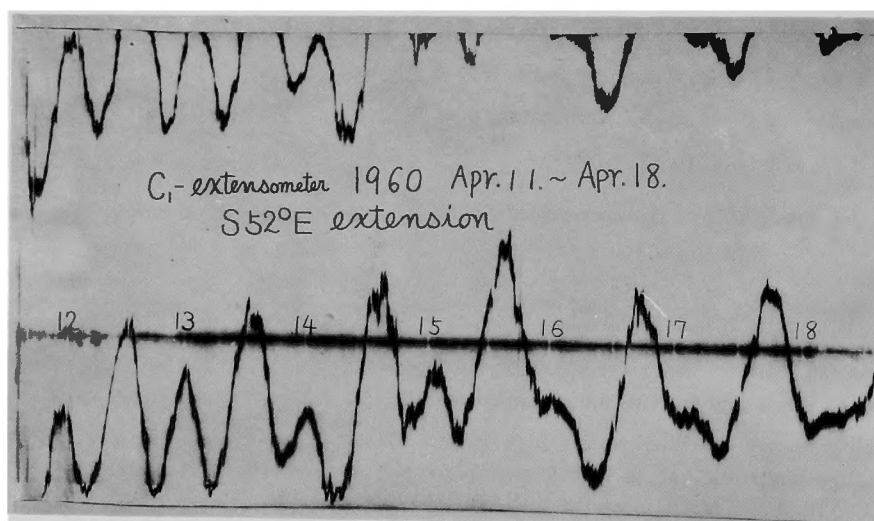
Photo. Photographic record of the tidal strain observed with the extensometer on the direction of S 52°E at Osakayama.
