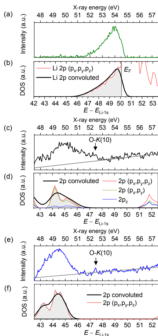
Figure 3 The experimental Li–K spectra for Li (a), \text{Li}_2\text{O}_2 (c), and \text{Li}_2\text{O} (e) using the SXES compared to the convoluted DOSs of occupied Li 2p states in Li metal (b), \text{Li}_2\text{O}_2 (d), and \text{Li}_2\text{O} (f) using HSE. Gray solid lines in panel (c) and (e) denotes linear background. Calculated energy is referenced to Li 1s centroid ( E_{\text{Li-1s}} ) where occupied Li 2p states below the Fermi energy and the VBMs are colored by gray. A comparison between the spectra and DOS using PBE is shown in Figure S3 in SI.
