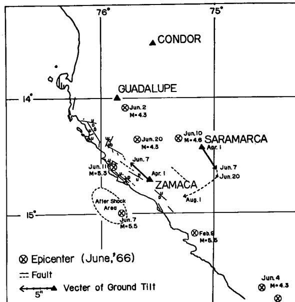
Fig. 9 Vector diagram of anomalous ground tilts at Zamaca and Saramarca related to the earthquake on June 7, 1966, and distribution of faults in the Ica region.
