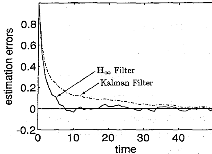
(a) E\{v_k^2\} = 0.01
