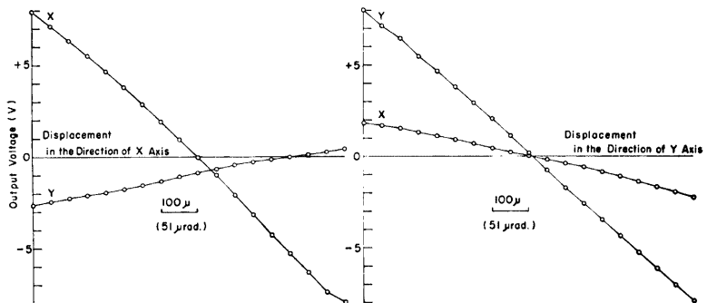
Fig. 8. Output voltage versus tilt (D/L). The displacement was given at the top of the casing pipe using a micrometer and sliding device. A cross-talk between X and Y appears.
