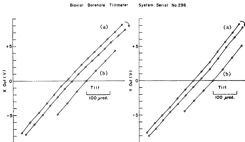
Fig. 9. Output voltage versus tilt.
