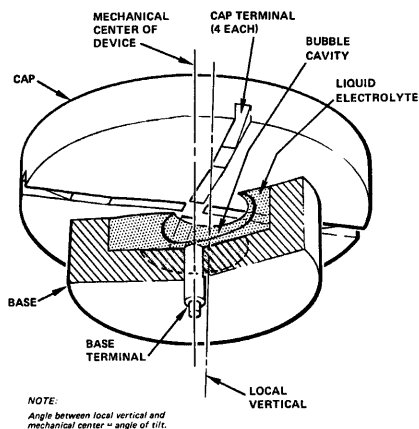
Fig. 1. Sensor assembly of a biaxial borehole tiltmeter (TM-1B, KINEMATRICS).
