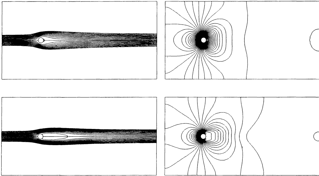
Figure 2: Streamlines (left, [-1, 1; 0.1] ) and pressure contours (right, [-1, 1; 0.02] ) of the stationary solution (u_h^*, p_h^*) for Re = 10 (top) and 100 (bottom).
