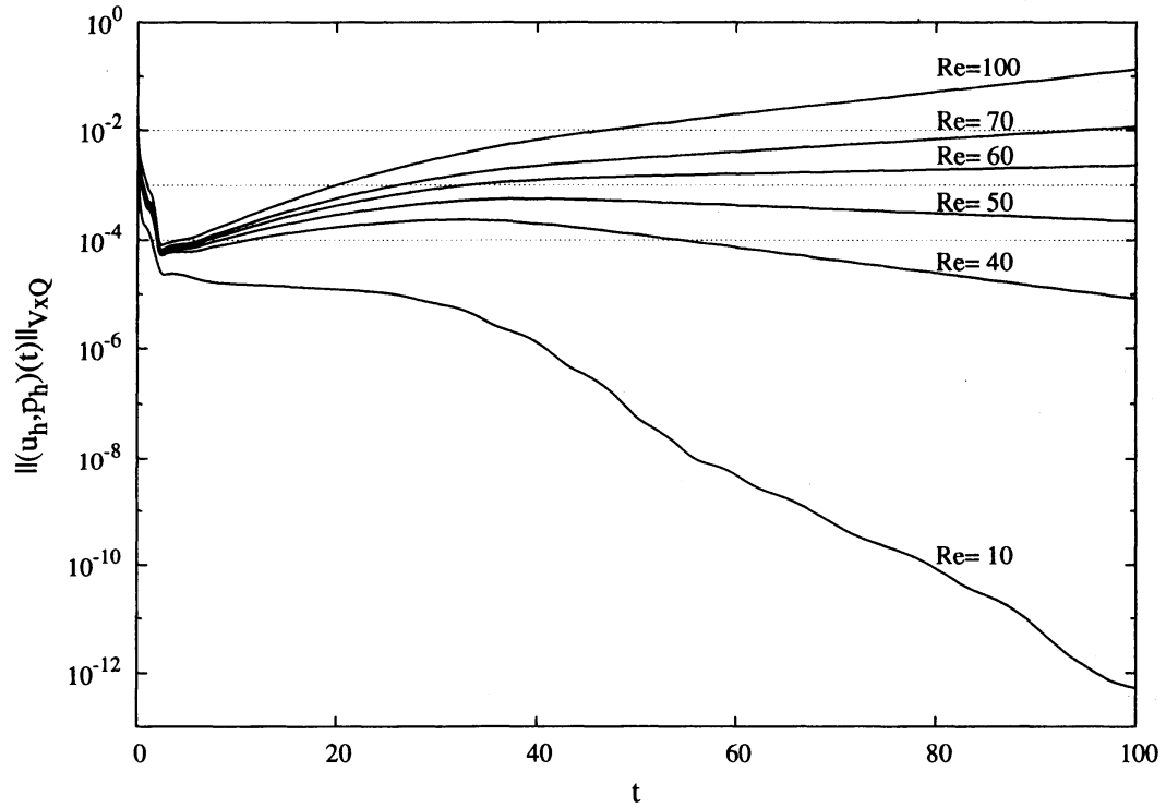
Figure 3: Graphs of \|(u_h, p_h)(t)\|_{V \times Q} vs. t for Re = 10, 40, 50, 60, 70 and 100 .
