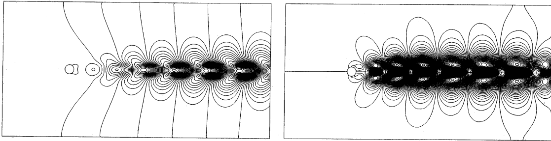
Figure 4: Streamlines (top, [-0.02, 0.02; 0.001] ) and pressure contours (bottom, [-0.003, 0.003; 0.0001] ) of (u_h, p_h)(t = 100) for Re = 100 .
