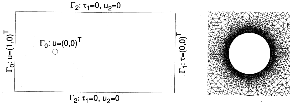
Figure 1: The domain \Omega with the boundary conditions for the Navier-Stokes equations (left) and the used triangular mesh around the cylinder (right).
