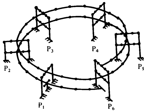
(a) Model of Senbonmatsu-Ohashi Bridge
