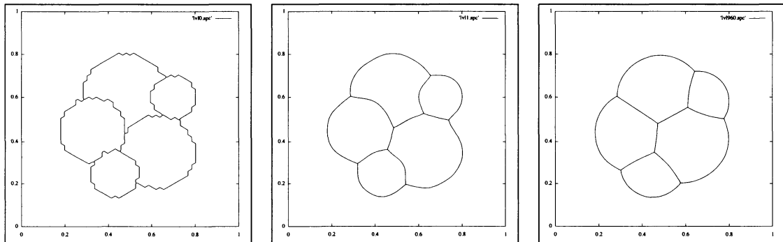
Figure 4: The initial condition, evolution after \Delta t , and the stable configuration.
