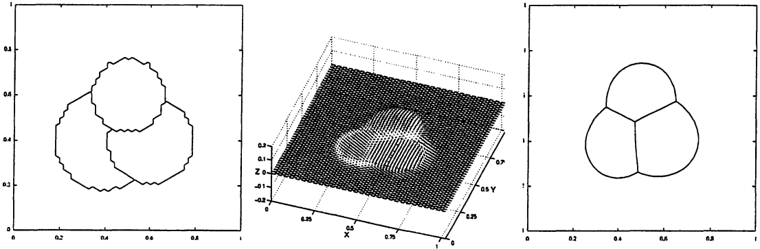
Figure 2: (Left) The initial condition. (Center) An instant in time of the vector-valued heat equation. (Right) The corresponding interfaces.
