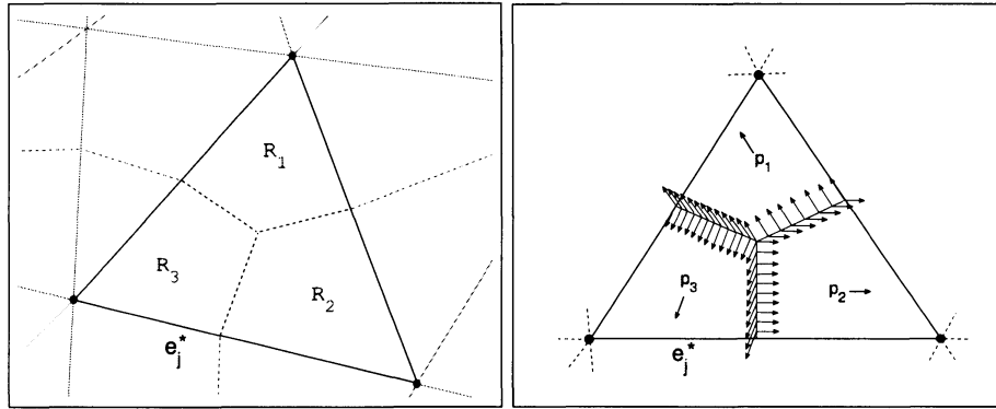
Figure 3: (Left) Three regions inside an indicated element. (Right) Vectors inside the element after thresholding.
