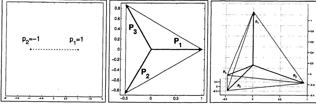
Figure 1: (Left) The 2-phase regular simplex. (Center) The 3-phase regular simplex. (Right) The 4-phase regular simplex.
