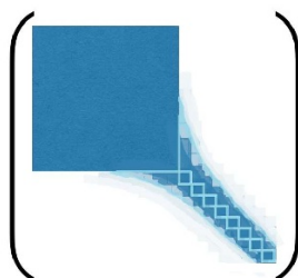
Figure 7. A more precise representation of the shape of the matrices describing a small black hole. In addition to the elements shown in (3.1), there is some ‘fuzziness’ which describes short open strings stretched between nearby D-branes. The light blue lines indicate where the blocks would be if the matrix were block diagonal. The color refers to the magnitude of the matrix elements, darker blue implying a larger magnitude.
