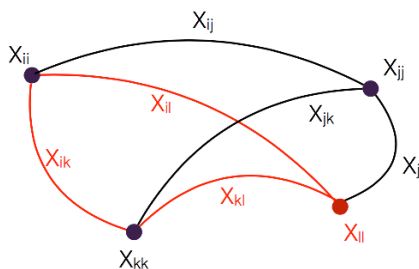
Figure 4. X_{M_1,ik}X_{M_2,kl}X_{M_3,ll}X_{M_4,li} in \text{Tr}(X_{M_1}X_{M_2}X_{M_3}X_{M_4})|Vac\rangle .
