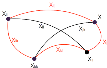
Figure 3. X_{M_1,ik}X_{M_2,kl}X_{M_3,lj}X_{M_4,ji} in \text{Tr}(X_{M_1}X_{M_2}X_{M_3}X_{M_4})|Vac\rangle .
