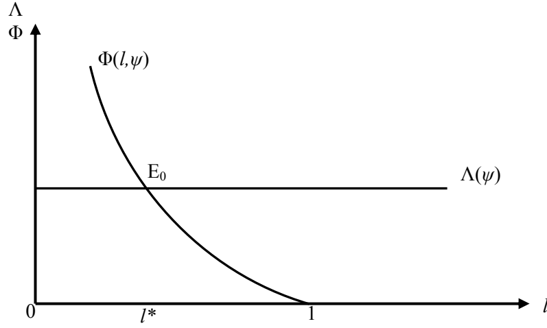
Figure 1: Existence of steady state under \psi(1-\nu)<\nu .
