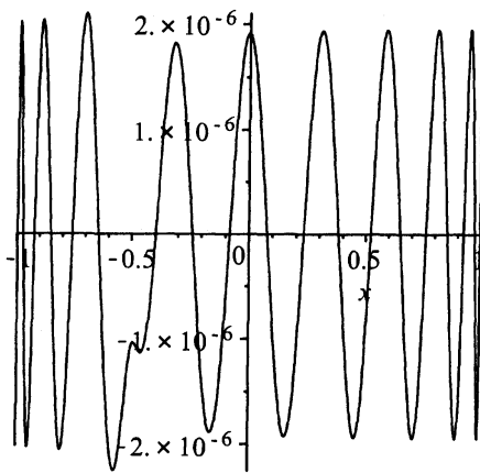
Figure 7: The approximate Tchebycheff function for m = 20 , w(x) = (x + 0.5)^2 + 0.001
