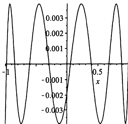
Figure 4: The approximate Tchebycheff function for m = 10 , w(x) = e^x
