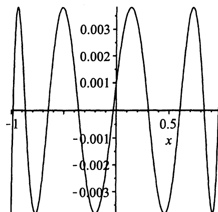
Figure 2: The approximate Tchebycheff function for m = 10 , w(x) = (1-x)^{1/2}(2+x)^{1/2}
