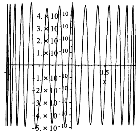
Figure 8: The approximate Tchebycheff function for m = 32 , w(x) = (x + 0.5)^2 + 0.001
