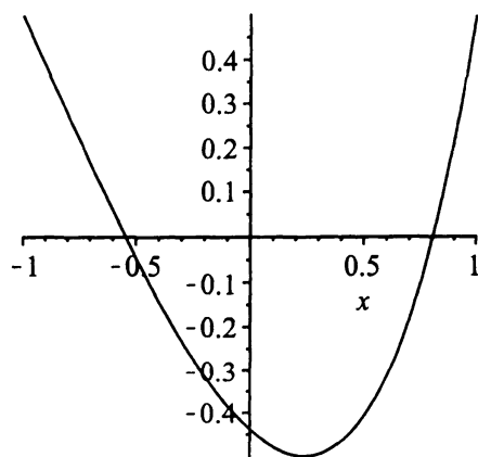
Figure 3: The approximate Tchebycheff function for m = 3 , w(x) = e^x
