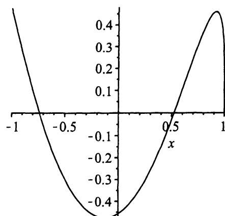
Figure 1: The approximate Tchebycheff function for m = 3 , w(x) = (1-x)^{1/2}(2+x)^{1/2}
