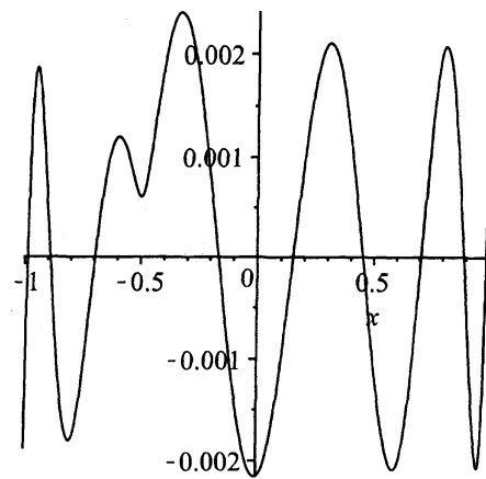
Figure 6: The approximate Tchebycheff function for m = 10 , w(x) = (x + 0.5)^2 + 0.001
