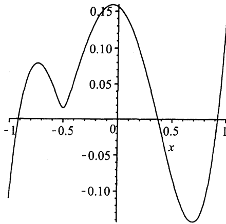
Figure 5: The approximate Tchebycheff function for m = 4 , w(x) = (x + 0.5)^2 + 0.001
