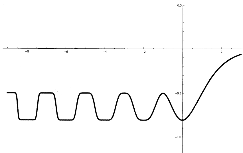
Figure 1: The graph of \tau(x)
