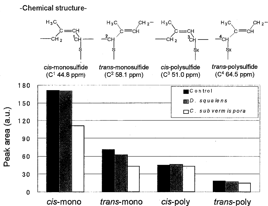
Figure I-7. Analysis of sulfide linkages in the NR sheets by DD/MAS solid state ^{13}\text{C} NMR: The rubbers were analyzed after cultivation of C. subvermispora and D. squalens for 250 days. *Control samples of the rubber were maintained for 250 days under the same culture conditions without inoculation by fungi.
