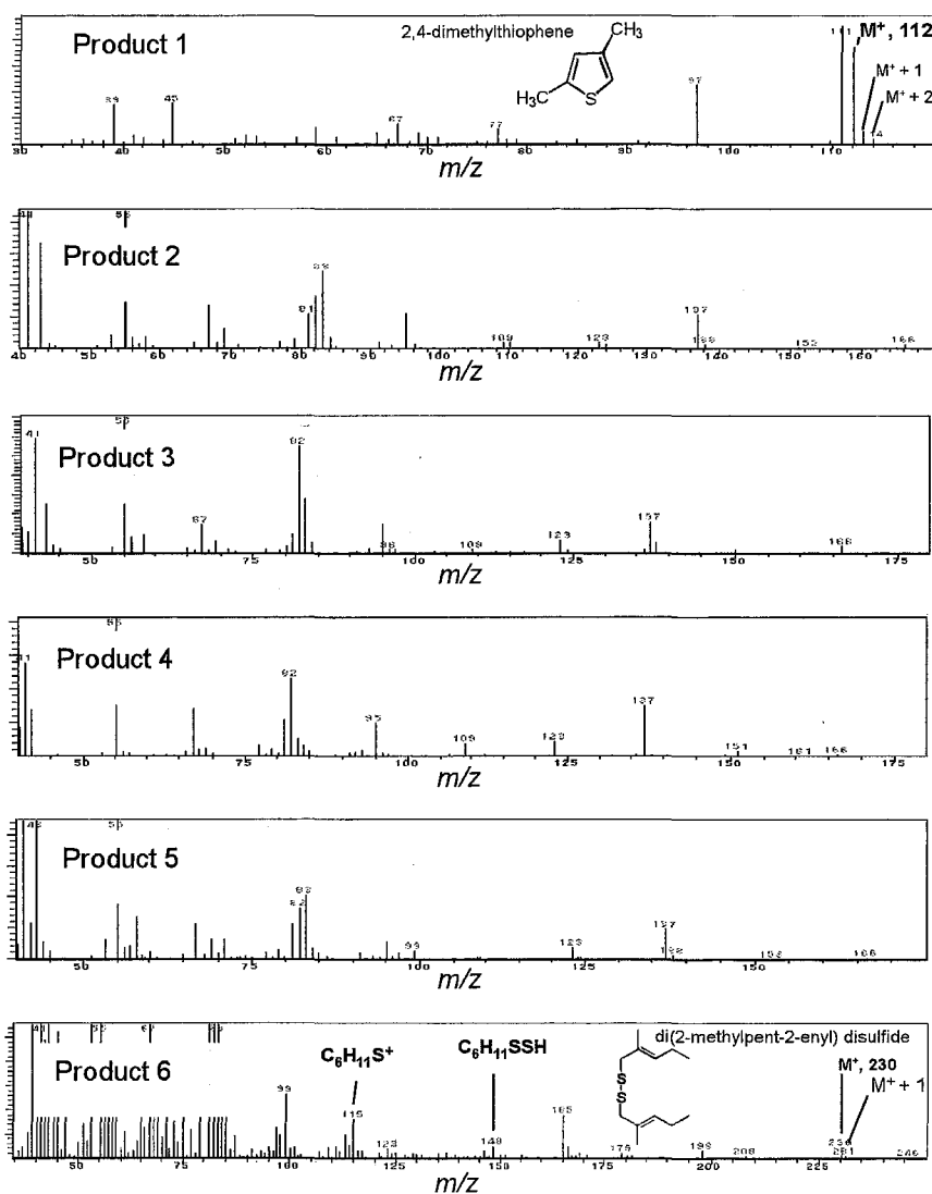
Figure III-3. Mass spectra of the products formed from the rubber model compound in LPO of 2E,4E-decadienal with MnP for 6 h.
