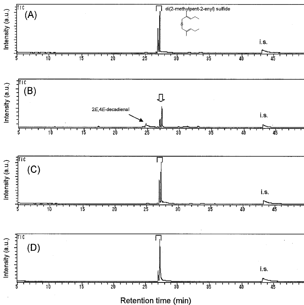
Figure III-2. Total ion chromatograms of the rubber model compound in LPO catalyzed by MnP for 6 h: (A) MnP without LPO; (B) LPO of 2E,4E-decadienal with MnP; (C) LPO of 2E-butene-1,4-dial with MnP; (D) LPO of 2E-butenal with MnP. i.s.; 0.5 mM fluoranthene.
