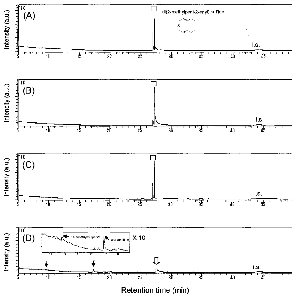
Figure III-1. Total ion chromatograms of the rubber model compound in LPO catalyzed by MnP for 6 h: (A) control without LPO of LA with MnP; (B) MnP; (C) LA autooxidation; (D) LPO of LA with MnP. i.s.; 0.5 mM fluoranthene.
