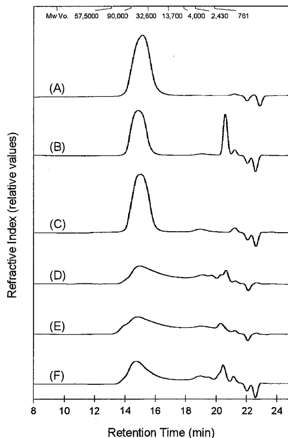
Figure II-3. GPC profiles of IR in the Mn(III)-catalyzed lipid peroxidation of unsaturated fatty acids for 48 h. (A) Control (original IR), (B) autooxidation of LA (- Mn(III)), (C) Mn(III) (-LA), (D) Mn(III)/LA, (E) Mn(III)/AA, (F) Mn(III)/LNA.
