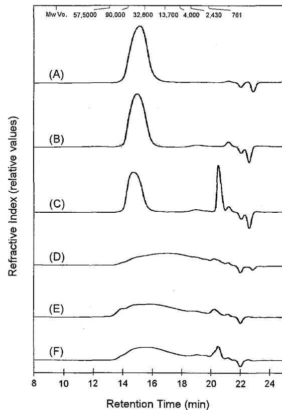
Figure II-1. GPC profiles of IR in the MnP-catalyzed lipid peroxidation of unsaturated fatty acids for 48 h. (A) Control, (B) MnP, (C) inactivated MnP/LA, (D) MnP/LA, (E) MnP/AA, (F) MnP/LNA.
