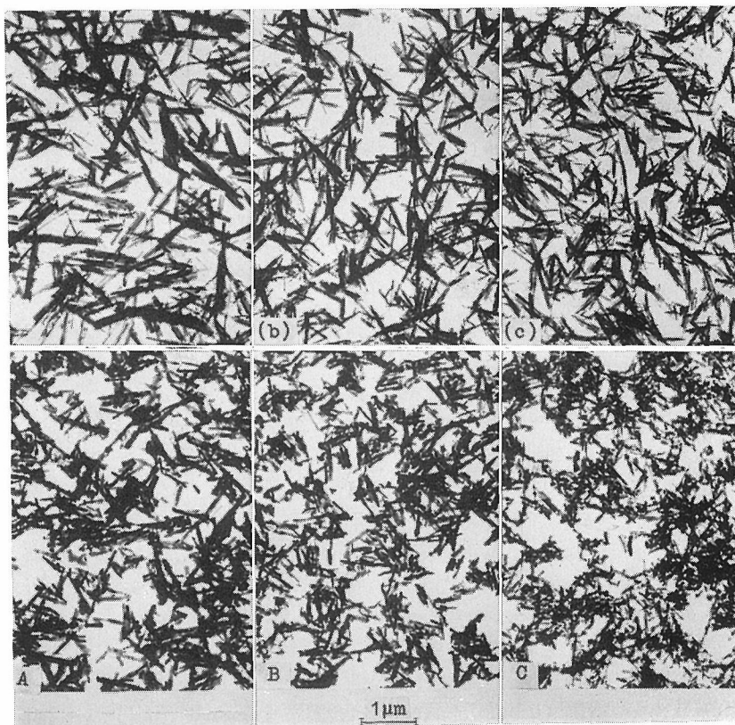
Fig. 5. TEM of \text{Fe}_3\text{O}_4 samples A, B and C (Table 3) prepared from the \alpha\text{-FeO}(\text{OH}) samples (each upper position).
