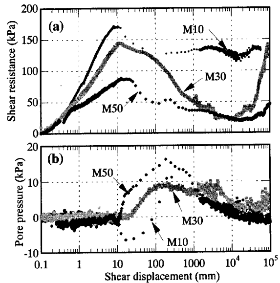
Fig.8 Results of naturally drained shear tests (Medium gear) on dense M10, dense M30, and “dense” M50 ( e = 0.87, 0.87 and 0.89 for M10, M30, and M50, respectively).
