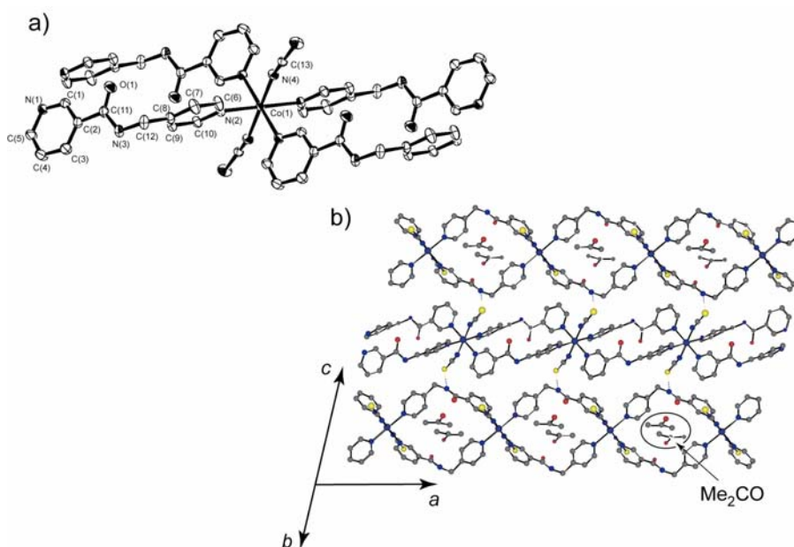
Figure 2. Crystal structure of \{[\text{Co}(\text{NCS})_2(4\text{-pcna})_2] \cdot 2\text{Me}_2\text{CO}\}_n ( R4 \equiv 2Me 2 CO). (a) ORTEP drawing of R4 \equiv 2Me 2 CO at the 30% probability level. Hydrogen atoms and acetone molecules are omitted for clarity. (b) Three repeated rhomboid typed chains which are connected by S---HN hydrogen bond, including acetone molecules.
