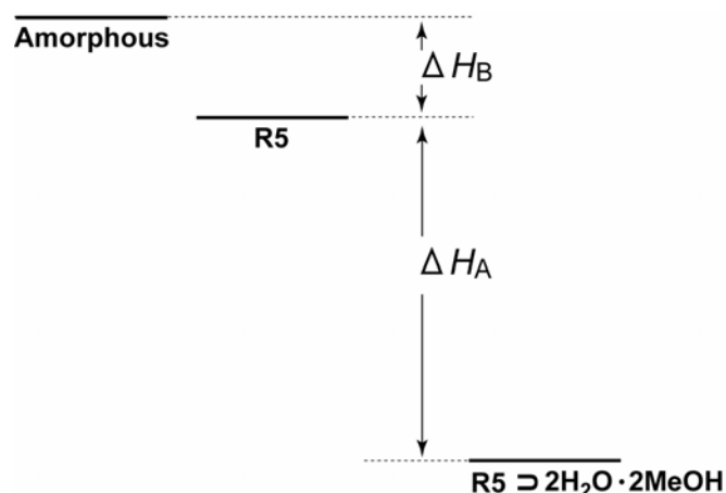
Figure 10. Schematic energy diagram for the solid-gas complexation of \mathbf{R5} \supset 2\mathbf{H_2O} \cdot 2\mathbf{MeOH} with methanol and water. Definitions are as follows: E_{\text{de}} are activation energy of acetone desorption in the processes of \mathbf{R5} \supset 2\mathbf{H_2O} \cdot 2\mathbf{MeOH} \rightarrow \mathbf{R5} . \Delta H_A and \Delta H_B are heat in the processes of \mathbf{R5} \supset 2\mathbf{H_2O} \cdot 2\mathbf{MeOH} \rightarrow \mathbf{R5} and \mathbf{R5} \rightarrow \text{Amorphous} , respectively.
