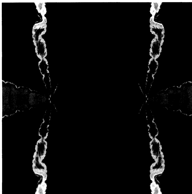
FIGURE 3. Bowditch's Q-condition: linear slice
