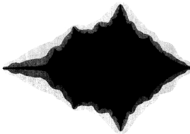
FIGURE 2. Primitive stable: Diagonal slice
