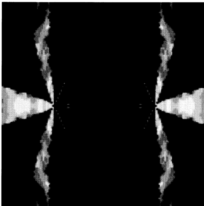
FIGURE 4. Primitive stable: linear slice
