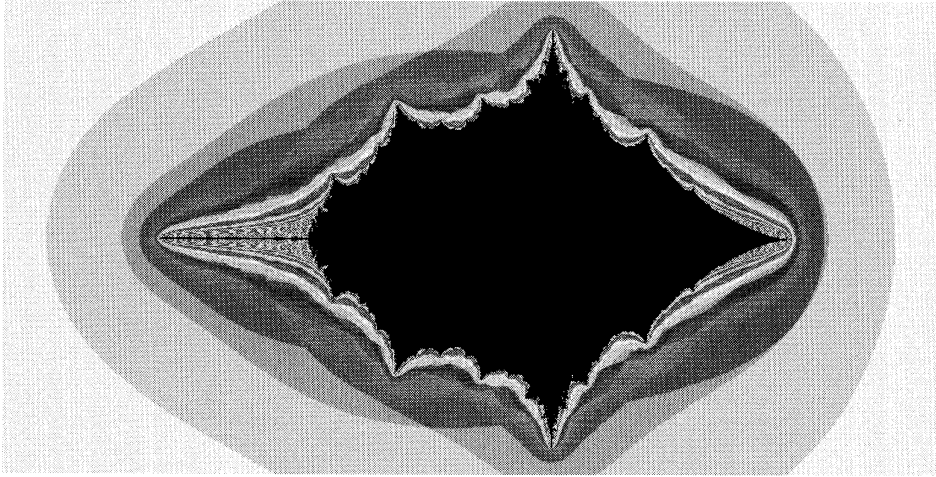
FIGURE 1. Bowditch's Q-condition: Diagonal slice
