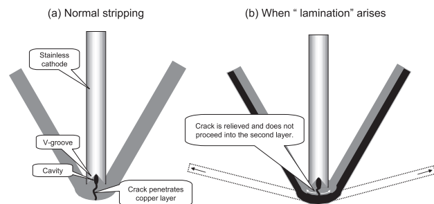
Fig. 1 In normal case (a), when stripping the electrodeposited copper, crack originating from the cavity at the V-groove at the bottom of stainless cathode, progresses and penetrates the copper layer smoothly by notch effect. When "lamination" arises (b), the growth of the crack is relieved at the interface of two copper layers before and after the power outage, and it becomes difficult to develop the cracking into the second layer.
