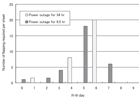
Fig. 2 Averaged number of flapping required for the stripping of electrolytic copper when the power outage for 6.5 or 34 h took place on the N-th day of cathode cycle (9 days in total) in Tamano refinery.
