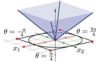
図 3: f(x) = \max\{|x_1|, |x_2|\} .
