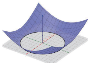
図 2: f(x_1, x_2) = \max\{\sqrt{x_1^2 + x_2^2} - 1, 0\} , C = \{(x_1, x_2) \mid x_1^2 + x_2^2 \leq 1\} .
