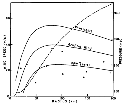
Fig. 1. An example of radial distribution of the gradient wind and the friction-free wind (FFW), in the directions perpendicular to the direction of typhoon motion. This example is for the data at 21 JST, Sept. 26th, 1959, in case of Typhoon 5915 (Isewan). A broken line represents radial pressure profile fitted with the Schloemer's formula. Open circles indicate observed surface winds in the right quadrant, and solid circles indicate those in the left quadrant.
