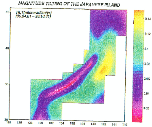
Fig. 1 The magnitude of tilting in the Japanese islands
