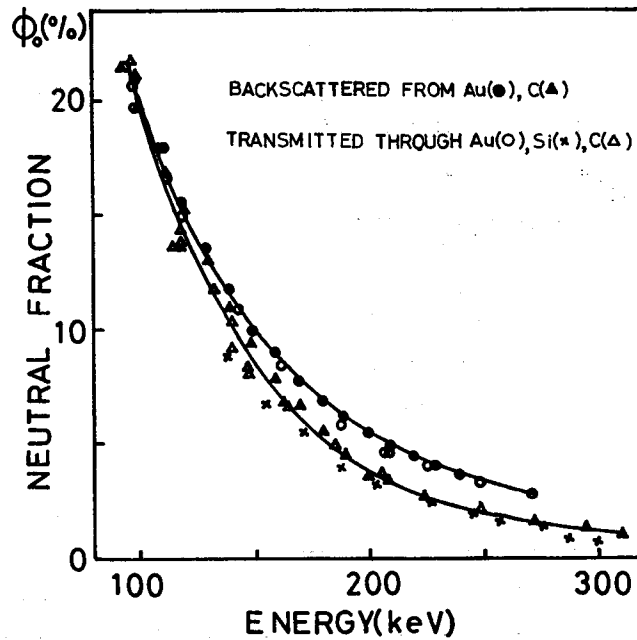
Fig. 3 Neutral fractions of proton beams backscattered from Au (●) and C (▲) targets and transmitted through Au (○) Si (×) and C (△) foils. Solid curves are drawn for eye fit.
