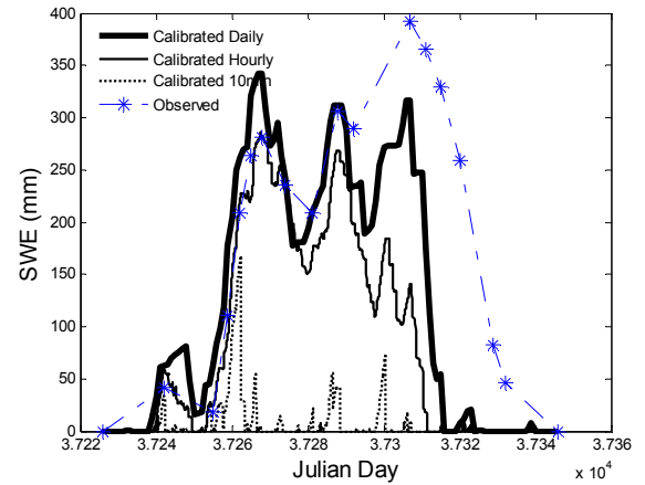
Fig. 4 Snow water equivalent ( SWE ) for the period of 1 December 2001 to 31 March 2002 calculated using the calibrated enhanced temperature-index method. Calibrated Hourly used hourly data.
