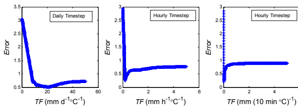
Fig. 5 Sensitivity of the temperature-index model to the temperature-factor ( TF ) considering different time scales. Error is the average relative error.
