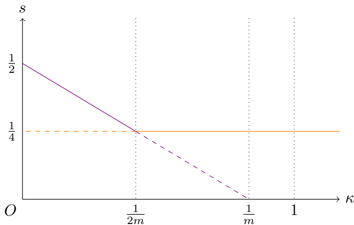
Figure 1. Sharp smooth regularity depending on \kappa when m > 1
