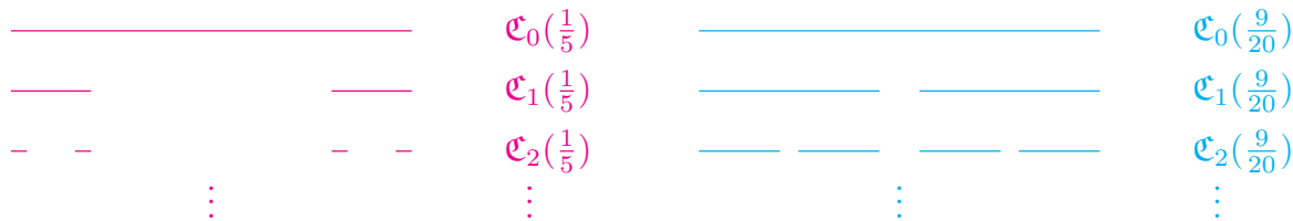
Figure 2. Each generation of pre-Cantor sets associated with \mathfrak{C}(\frac{1}{5}) and \mathfrak{C}(\frac{9}{20})
