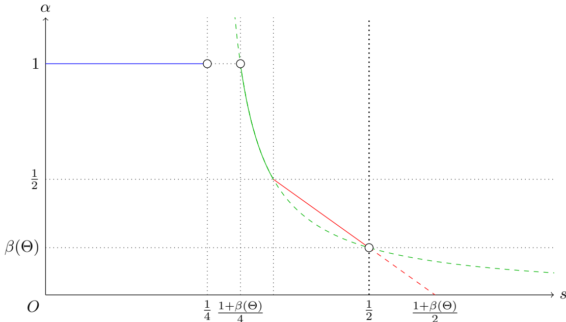
Figure 3. Graph of \alpha = 1 when s \in [0, \frac{1}{4}) and \alpha = \min\{\frac{\beta(\Theta)}{4s-1}, 1 + \beta(\Theta) - 2s\} when s \in (\frac{1 + \beta(\Theta)}{4}, \frac{1}{2})
