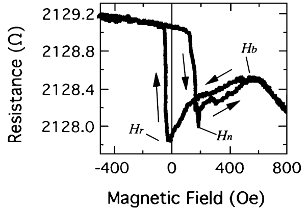
Figure 2. The minor loop of the magnetoresistance of a NiFe(200Å) wire with three CoSm(400Å) pads at 5 K.
