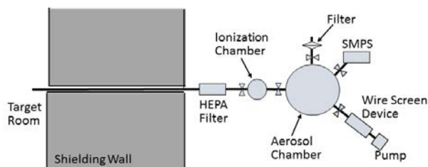
Fig. 1 Experimental Setup for Sampling of the irradiated air from the target room
