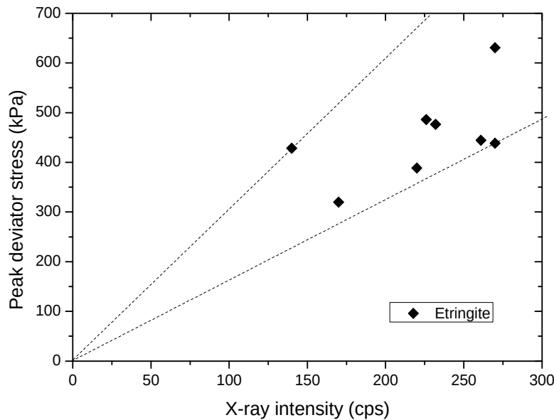
Fig. 3.28 Variation of peak deviator stress with XRD diffraction intensity of ettringite
