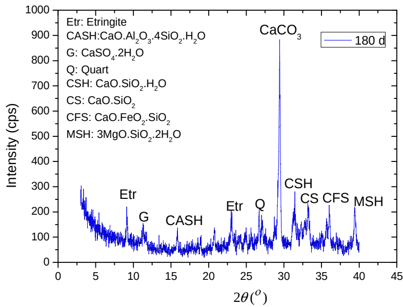
Fig. 3.19 XRD results for waste mixture samples cured for 180 days in simulated leachate
