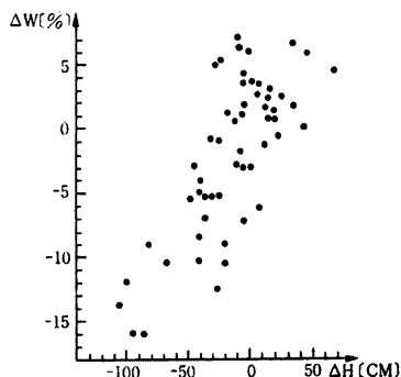
Fig. 4. Relationship between change of level of Caspian Sea ( \Delta H ) and that of wheat yield in the United States of America ( \Delta W ), after Budyko 1) .
