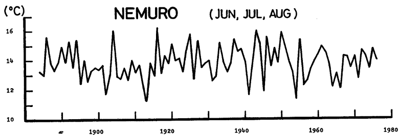
Fig. 1. 3-month mean of surface air temperature of June, July and August at Nemuro ( 43^{\circ}20'N , 145^{\circ}35'E ).
