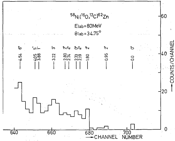
Fig. 6, Energy spectrum of the ^{58}\text{Ni}(^{16}\text{O}, ^{12}\text{C})^{62}\text{Zn} reaction at the incident energy E_{\text{lab}}(^{16}\text{O}) = 80 MeV and the measured angle \theta_{\text{lab}}(^{12}\text{C}) = 34.75^\circ .
