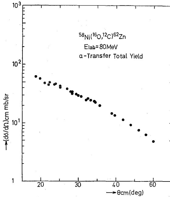
Fig. 7, Measured cross section angular distribution of the ^{58}\text{Ni}(^{16}\text{O}, ^{12}\text{C})^{62}\text{Zn} reaction at the incident energy E_{\text{lab}}(^{16}\text{O}) = 80 MeV leading to the continuum state in the ^{62}\text{Zn} .
