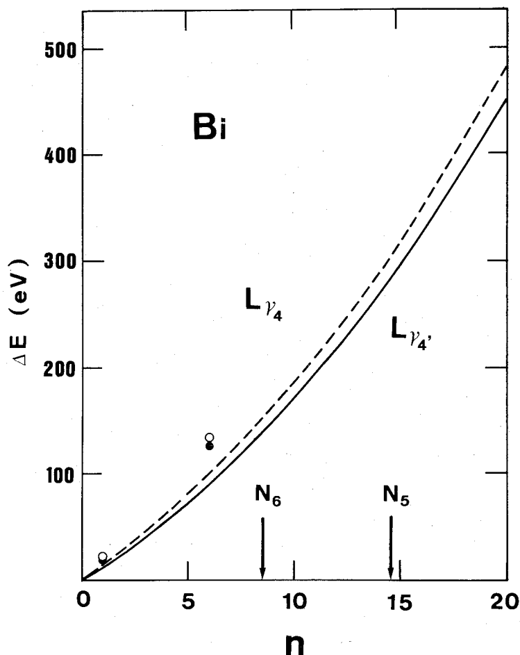
Fig. 1. Energy shift, \Delta E , of L_{\gamma} x rays as a function of the number of N-shell vacancies, n . The solid line indicates the shift for L_{\gamma_4'} x rays, while the dashed line represents the shift for L_{\gamma_4} x rays. The positions where the N_5 and N_6 shells start to be removed are shown by the arrows. The solid and open circles indicate the values when the N_5 electrons are removed instead of the N_7 electrons.
