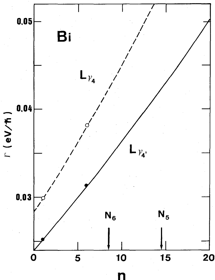
Fig. 2. Transition probability, \Gamma , of L_{\gamma} x rays as a function of n . See caption of Fig. 1.
