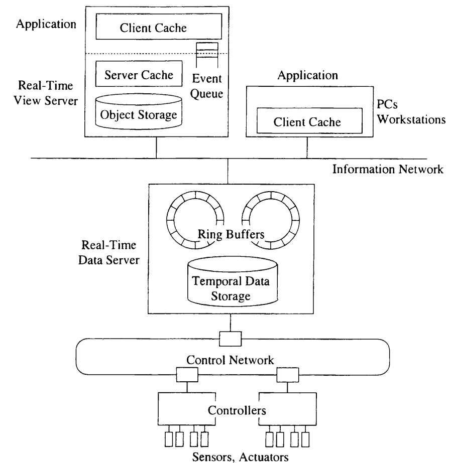
Figure 3.2: Two Layered Architecture for Plant Monitoring Database Systems
