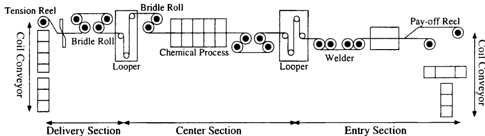
Figure 5.13: A Typical Steel Process Line
